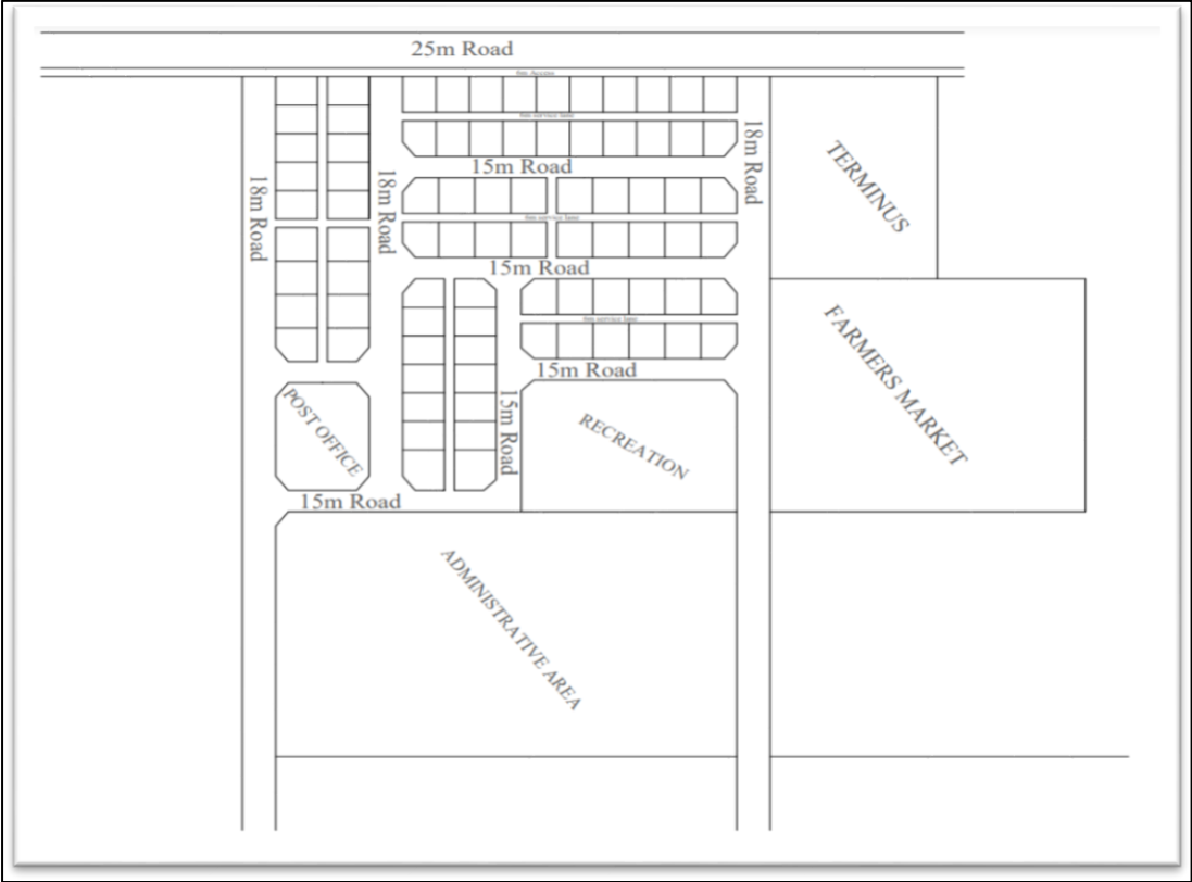
Figure 43: Road Hierarchy in Commercial Areas
