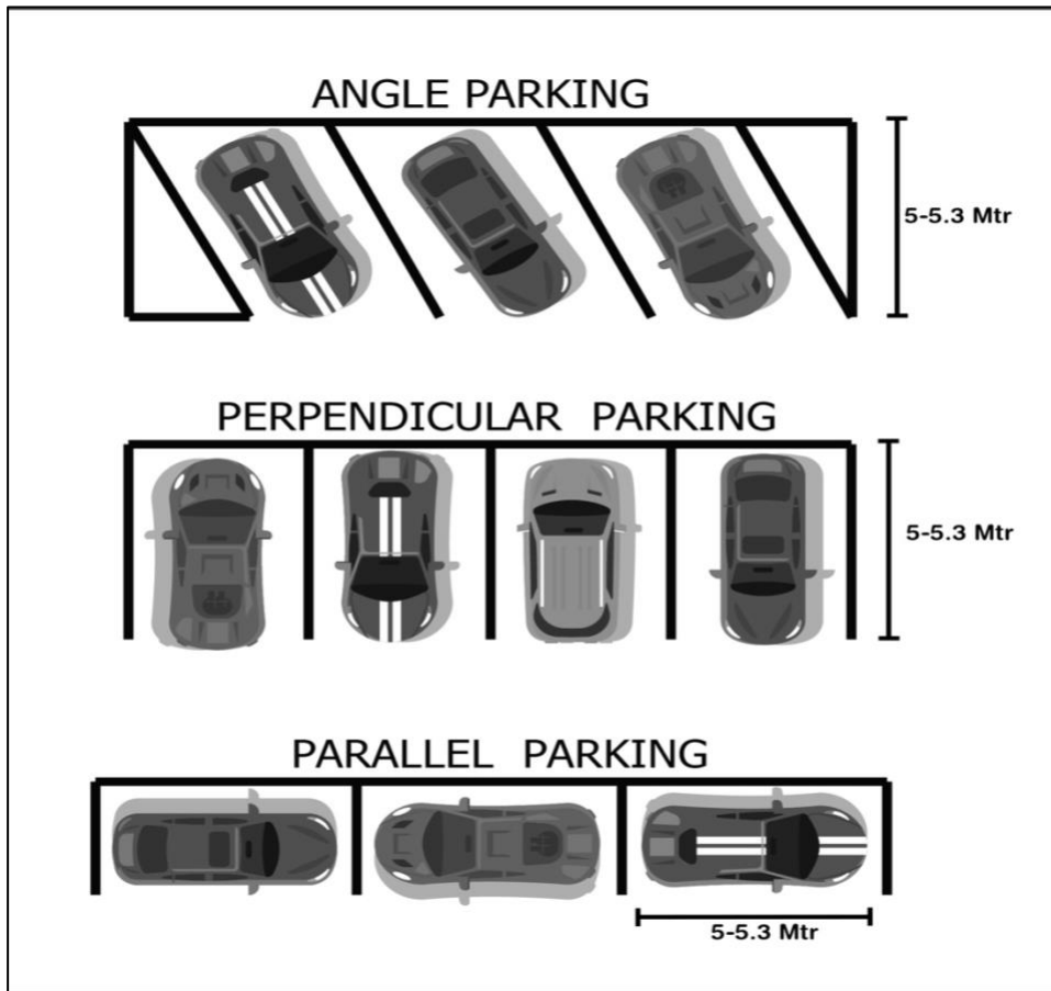
Figure 25: Types of parking
