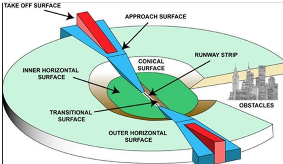
Figure 29: Obstacle Limitation Surface (OLS)
