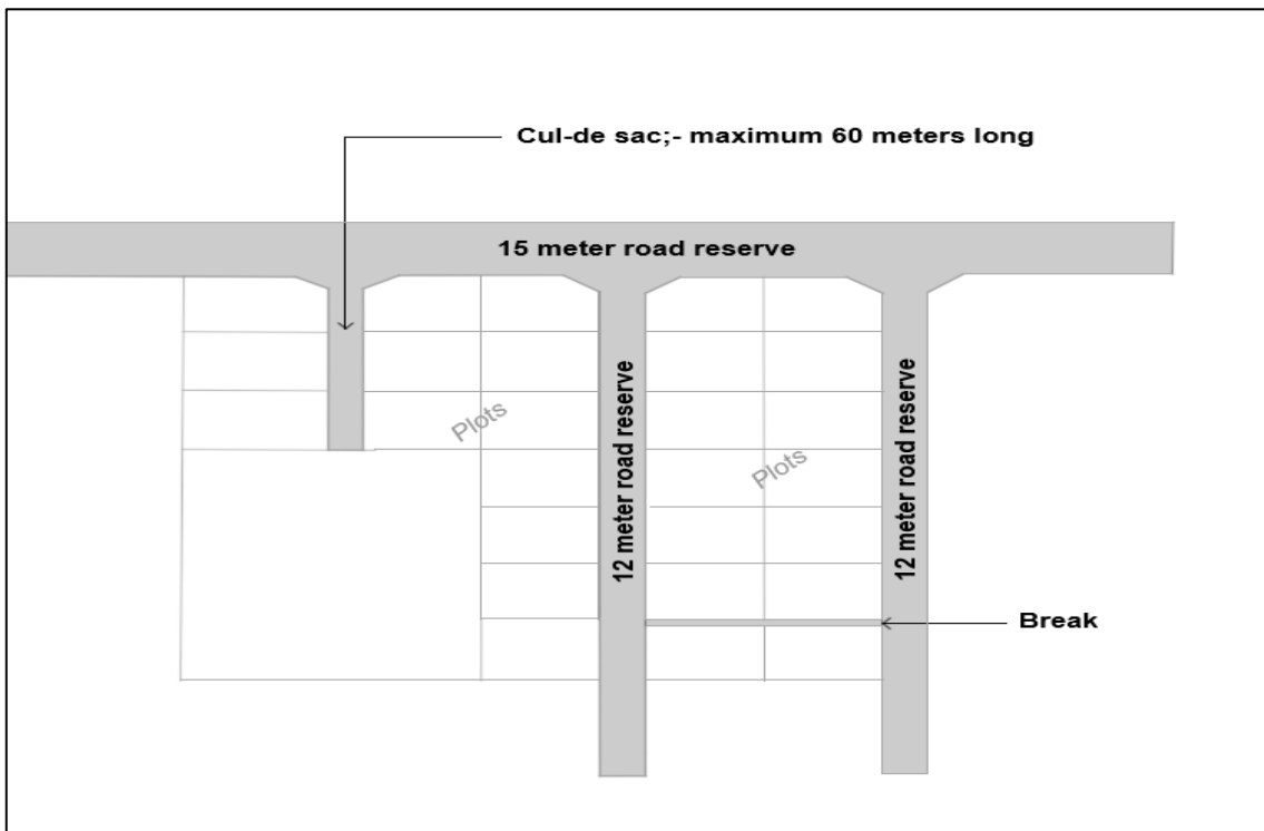
Figure 42: Access in Residential Areas
