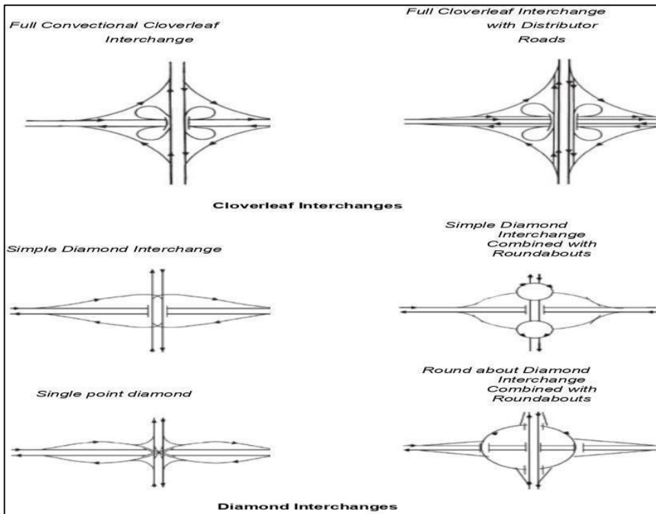
Figure 24: Road Interchange
